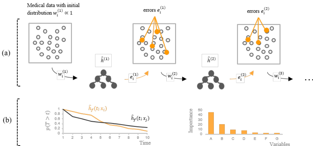
Figure 1: Overview of our boosting procedure for survival analysis. (a) illustrates the training procedure of our model: the second survival tree \hat{h}^{(2)} is trained on weighted samples w_i^{(2)} of the patient data, depending on the predictive performance of previous survival trees on individual patients (in this case through errors e_i^{(1)} of tree \hat{h}^{(1)} ). (b) shows the final output of the ensemble: we combine predictions (individual survival functions) of learned trees \hat{h}^{(1)}, \hat{h}^{(2)}, \dots to produce flexible estimates of survival (left) and investigate influential covariates in the tree construction which results in a measure of covariate importance (right).
