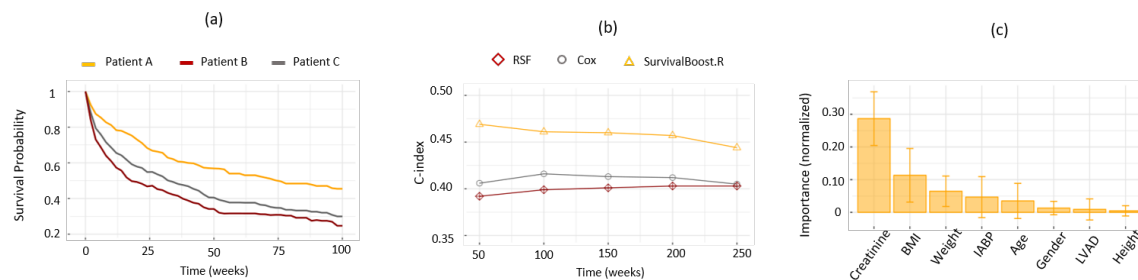
Figure 2: Panel (a) shows an illustration of predicted survival curves with SurvivalBoost.R for three selected patients from the UNOS data set with different levels of Creatinine. In panel (b) we show predictive performance of SurvivalBoost.R, RSF and Cox models on a challenging sub-population of UNOS. In panel (c) we show predicted covariate importance for the UNOS data according to SurvivalBoost.R.
