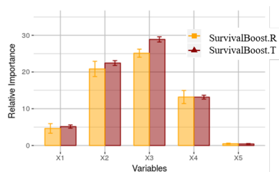
Figure 3: Predicted covariate importance for SurvivalBoost.R and SurvivalBoost.T.
